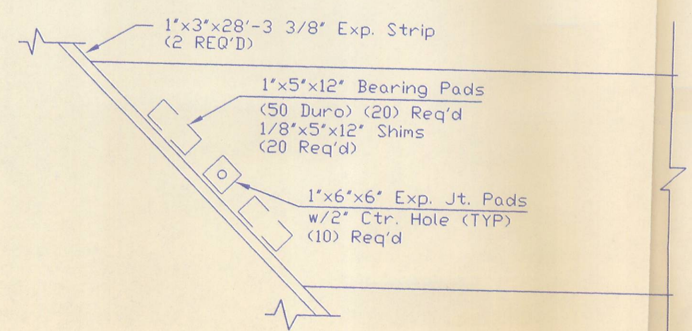
BEARING PAD PLACEMENT DETAIL
